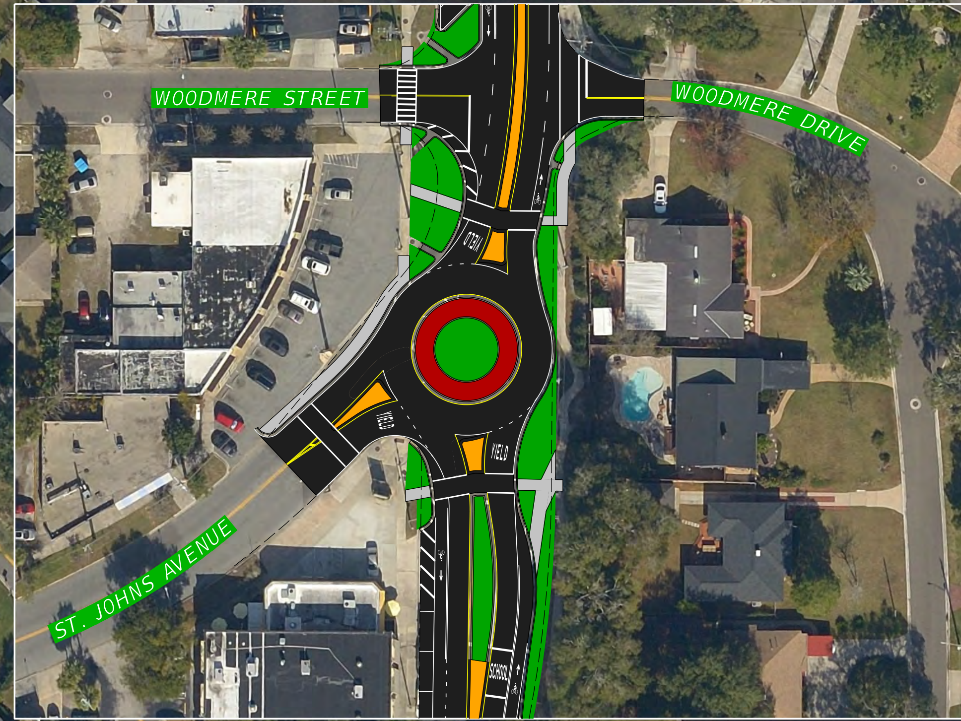
OPTION 2 WITHOUT RECTANGULAR RAPID FLASHING BEACON ASSEMBLY ON ST. JOHNS AVENUE
