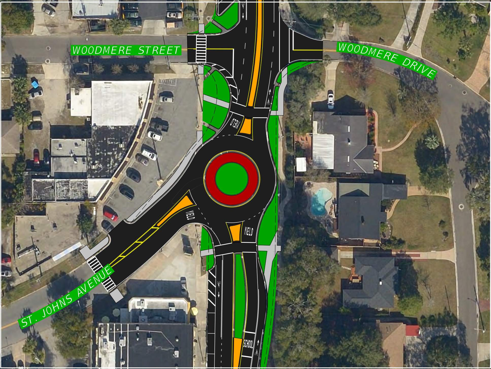
OPTION 1 WITH RECTANGULAR RAPID FLASHING BEACON ASSEMBLY ON ST. JOHNS AVENUE
